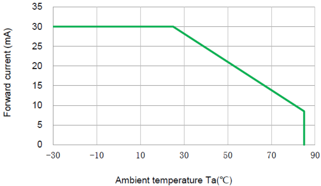
Fig.5 Forward current VS. Ambient temperature
